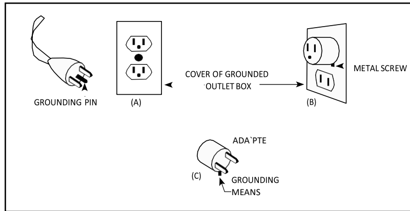
Figure: Outlet/Plug Grounding
