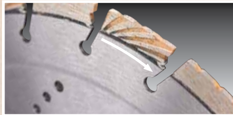
Alternating turbo segment for cut speed, and plain segment for life
